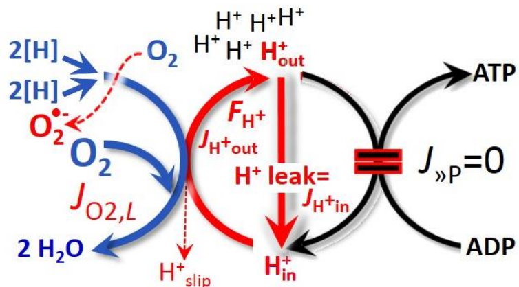
Fig. 5. LEAK state: Phosphorylation is arrested, J_{>>P}=0 , and oxygen flux, J_{O_2,L} , is controlled mainly by the proton leak, which equals J_{H^+in} , at maximum protonmotive force, F_{H^+} (See also Fig. 2).
