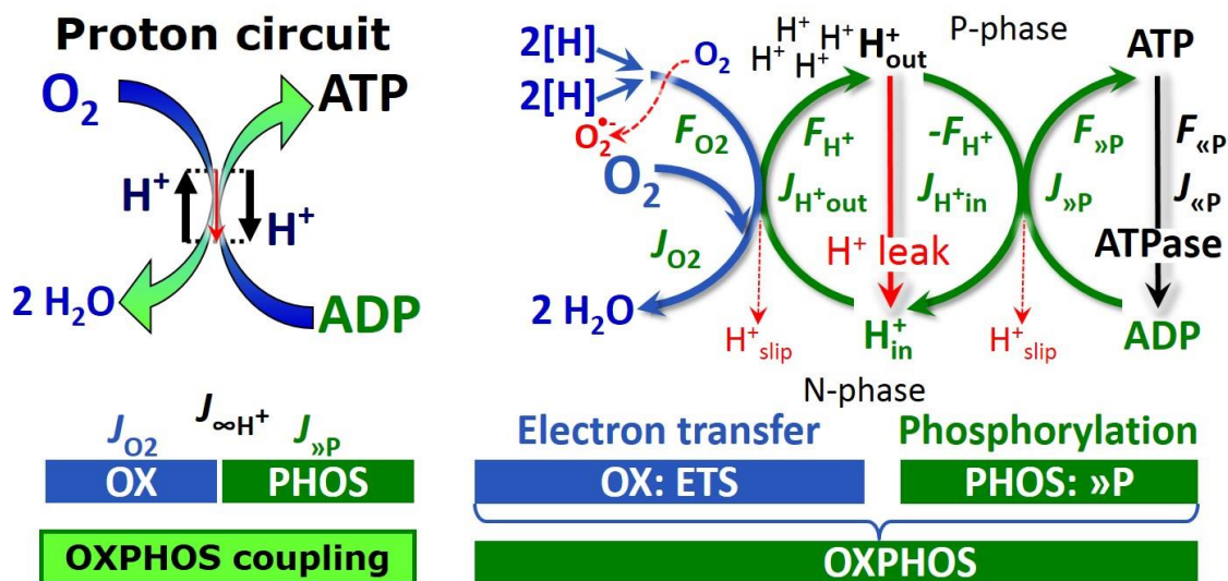
Fig. 2. The proton circuit and coupling in oxidative phosphorylation (OXPHOS). Oxygen flux, J_{\text{O}_2} , is coupled to the phosphorylation of ADP to ATP, J_{\text{»P}} , by the proton pumps of the electron transfer system, ETS, pushing the outward proton flux, J_{\text{H}^+\text{out}} , and generating the output protonmotive force, F_{\text{H}^+} . ATP synthase is driven by the input protonmotive force, -F_{\text{H}^+} , and inward proton flux, J_{\text{H}^+\text{in}} , to phosphorylate ADP to ATP. 2[\text{H}] indicates the reduced hydrogen equivalents of fuel substrates that provide the
